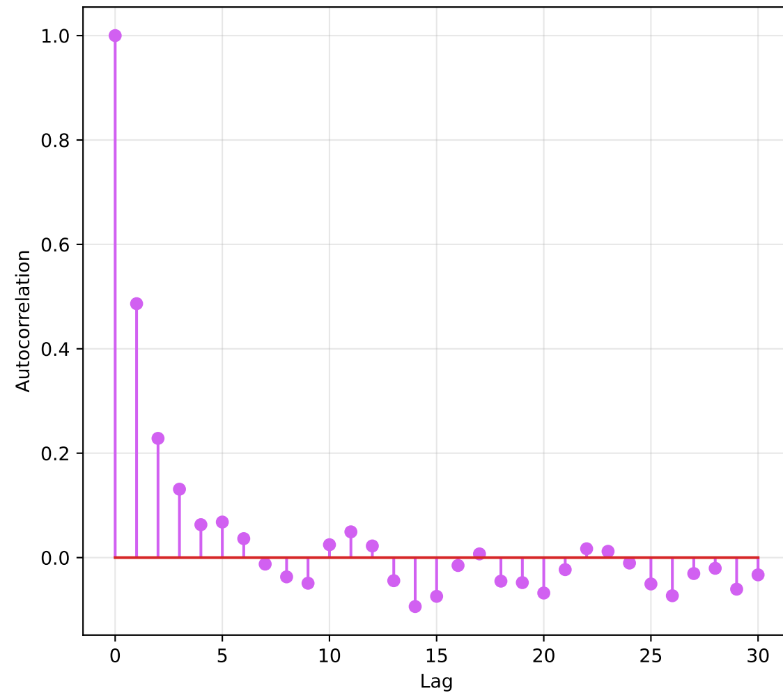
Autocorrelation: Random Walk
